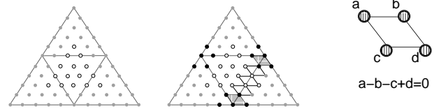
Figure 4: C^1 -conditions between two adjacent quintic Bézier patches.
